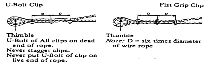
FIGURE 15-1 WIRE ROPE CLIPS
