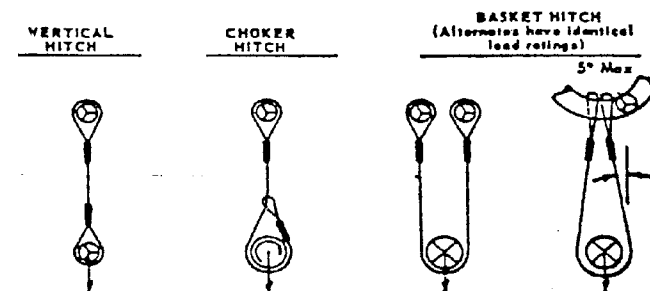
FIGURE 15-2 SLING CONFIGURATIONS
